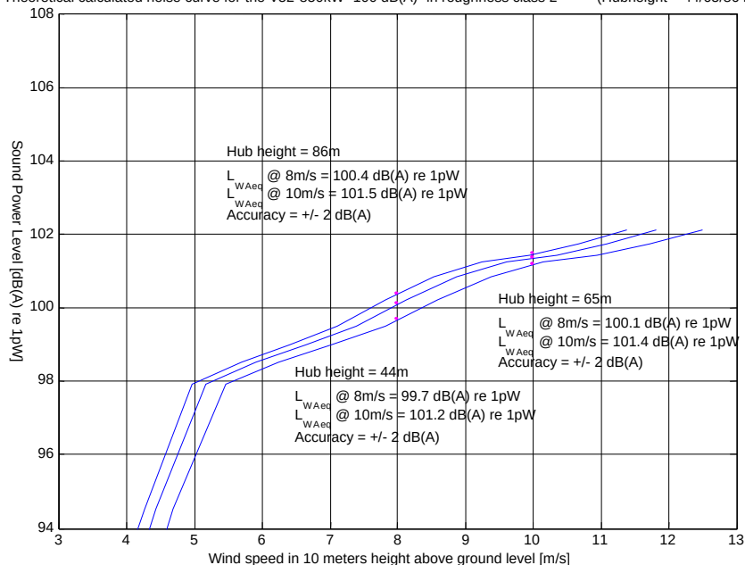
Theoretical calculated noise curve for the V52-850kW "100 dB(A)" in roughness class 2 (Hubheight = 44/65/86 m)
